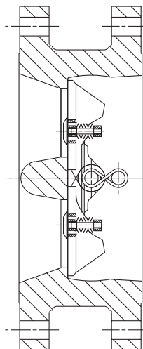
Schematic of a 32" 150lb Valve with APS.
